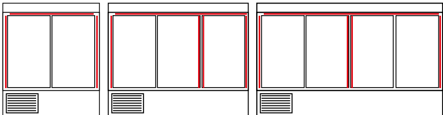
Red lines on diagrams show placement of LED lighting on EXPRESS CD Range
