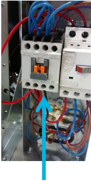
Modular units: red cable (second one) is the compressor cable
